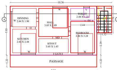
GROUND FLOOR PLAN (EAST FACING)
