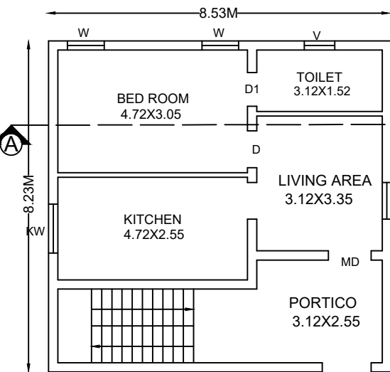
GROUND FLOOR PLAN (EXISTING)
