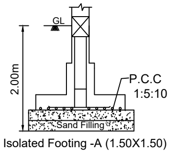
FOUNDATION DETAIL NOT TO SCALE
