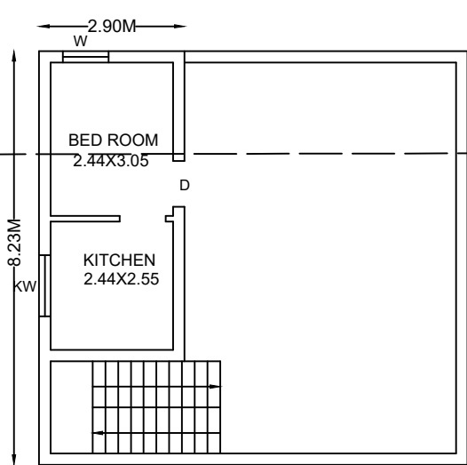
SECOND FLOOR PLAN (PROPOSED)
