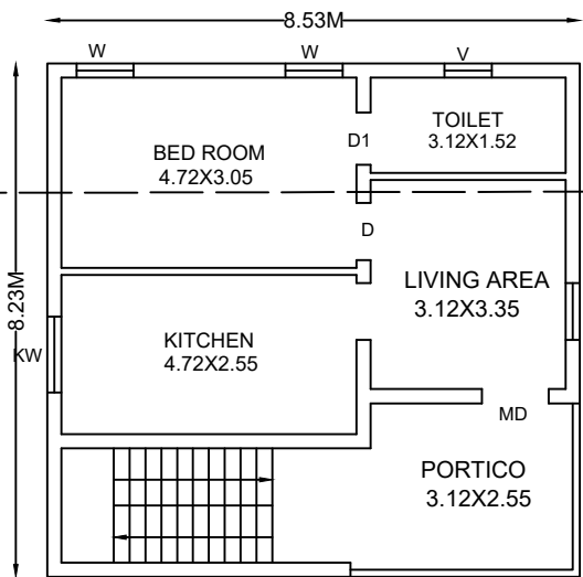
FIRST FLOOR PLAN (PROPOSED)
