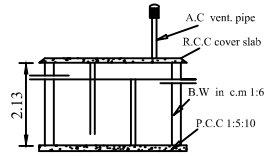
"S" TRAP DETAILS - IWC
