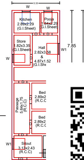
PLAN - G.F.
