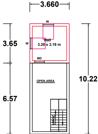
FIRST FLOOR PLAN & TERRACE FLOOR PLAN
