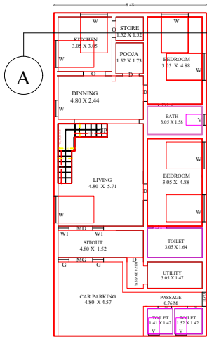
GROUND FLOOR PLAN (NORTH FACING)
