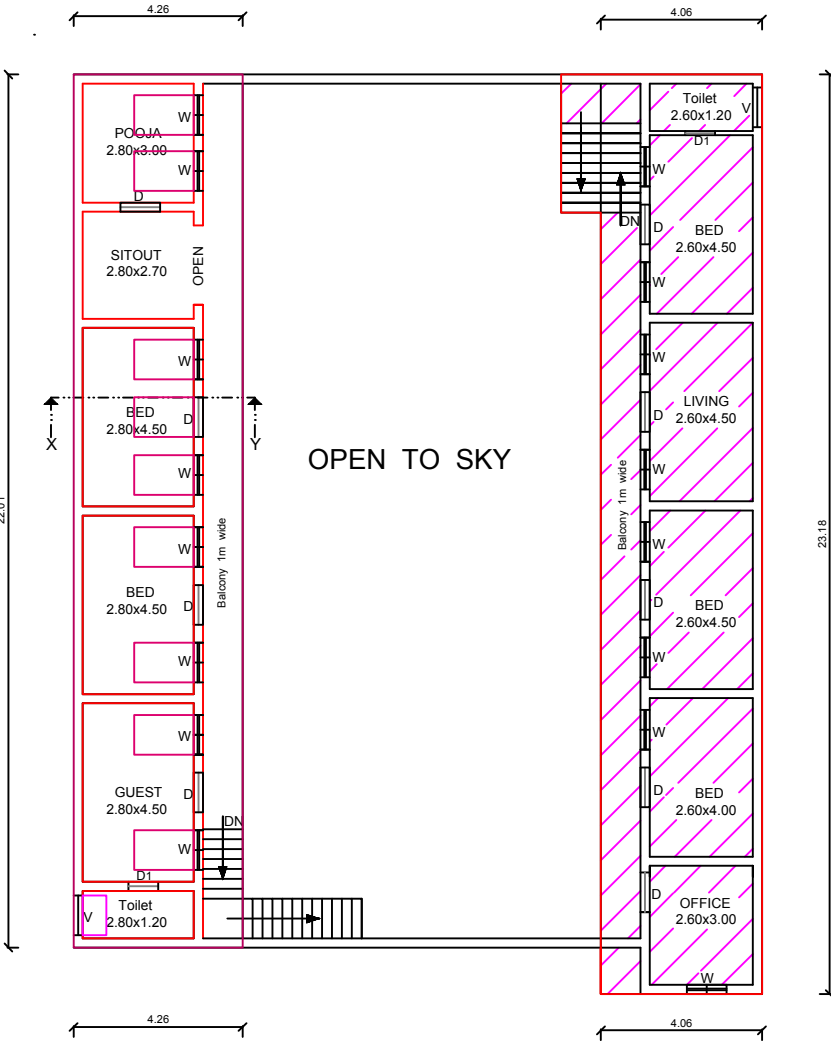
Pro.FIRST FLOOR PLAN FACING EAST
