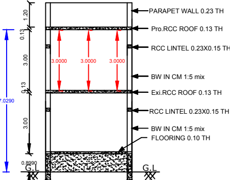
SECTION ON X-Y
