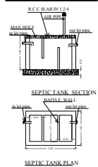
SEPTIC TANK DETAILS
