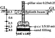
FOUNDATION DETAILS
