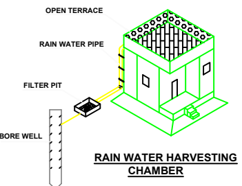
RAIN WATER HARVESTING CHAMBER
