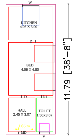
GROUND FLOOR PLAN ( NORTH FACING)
