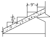
Staircase Detail Not To Scale
