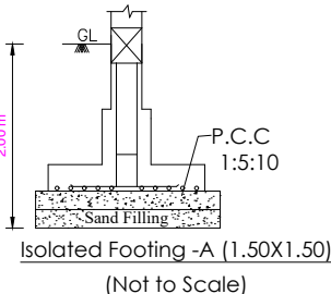
Isolated Footing -A (1.50X1.50) (Not to Scale)
