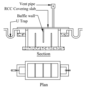
Waste Water Recycle Unit Not To Scale
