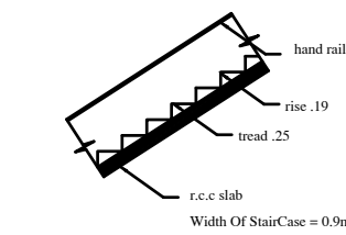
STAIRCASE DETAILS
