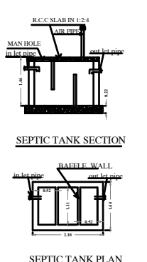
SEPTIC TANK PLAN
