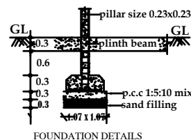
FOUNDATION DETAILS
