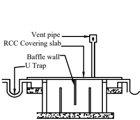
Waste Water Recycle Unit Not To Scale
