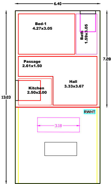
GROUND FLOOR PLAN (FACEING OF EAST)
