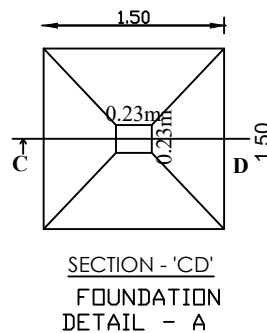
Isolated Footing -A (1.50X1.50) (Not to Scale)
