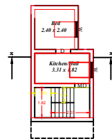
Proposed First Floor Plan
