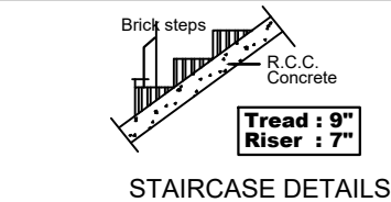
STAIRCASE DETAILS
