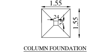
COLUMN FOUNDATION
