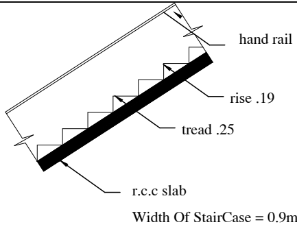
STAIRCASE DETAILS
