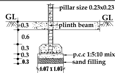
FOUNDATION DETAILS
