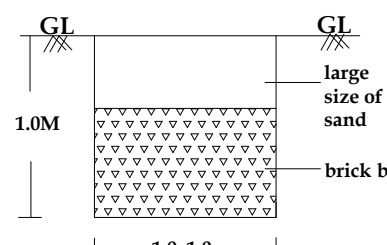
RAINWATER HARVESTING
