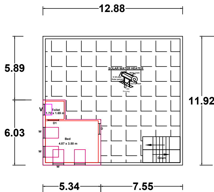
FIRST FLOOR & TERRACE FLOOR PLAN
