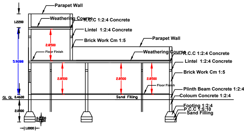
Section Section - AA
