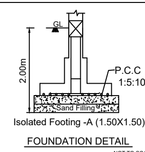
FOUNDATION DETAIL
