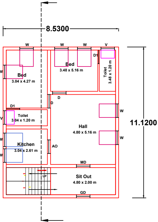
Ground Floor Plan (East Facing)
