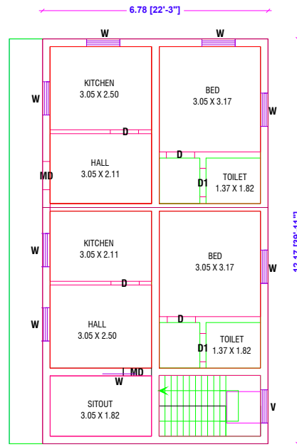
FIRST FLOOR PLAN [ NORTH FACING ]
