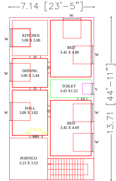
GROUND FLOOR PLAN NORTH FACING
