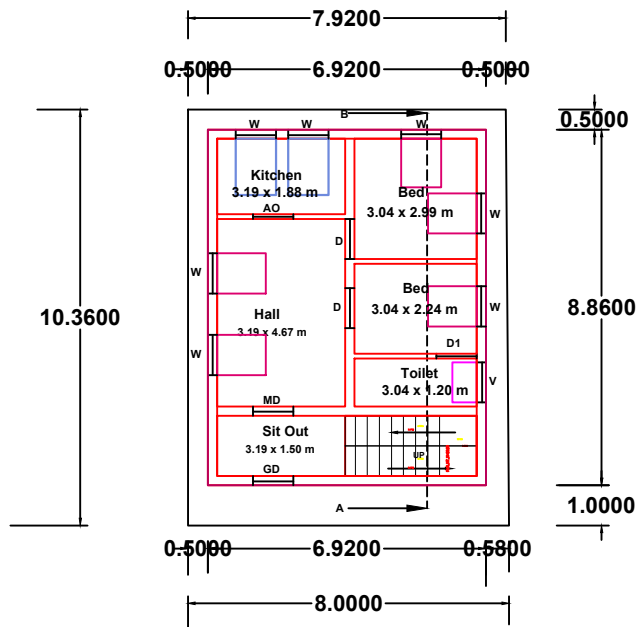
Ground Floor Plan North Facing
