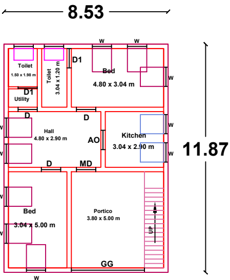
GROUND FLOOR PLAN (WEST FACING)
