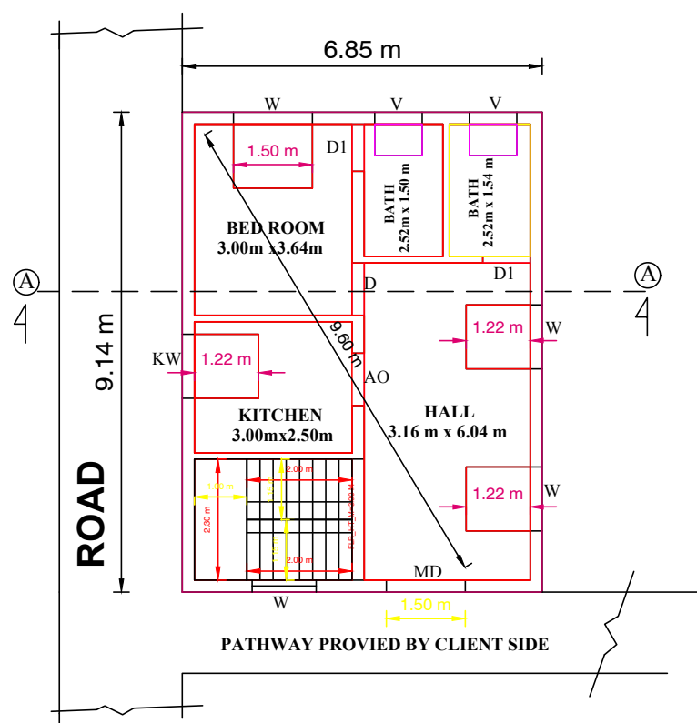
GROUND FLOOR PLAN [EAST FACING]
