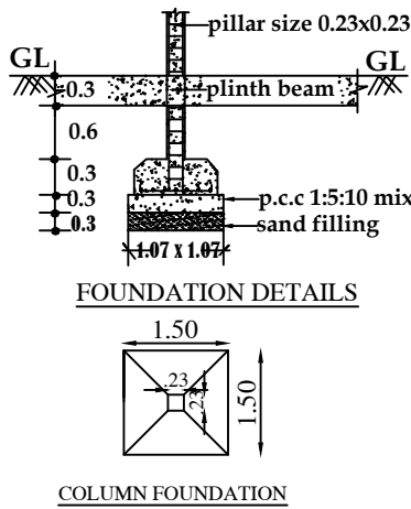
COLUMN FOUNDATION
