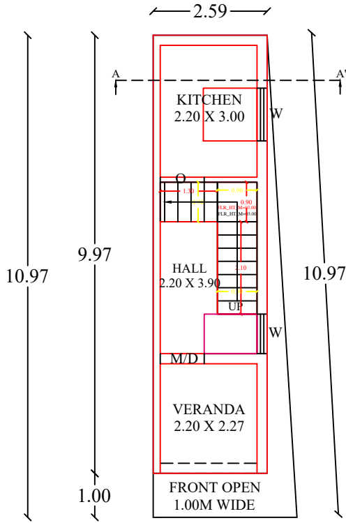
GROUND FLOOR PLAN (NORTH FACING)
