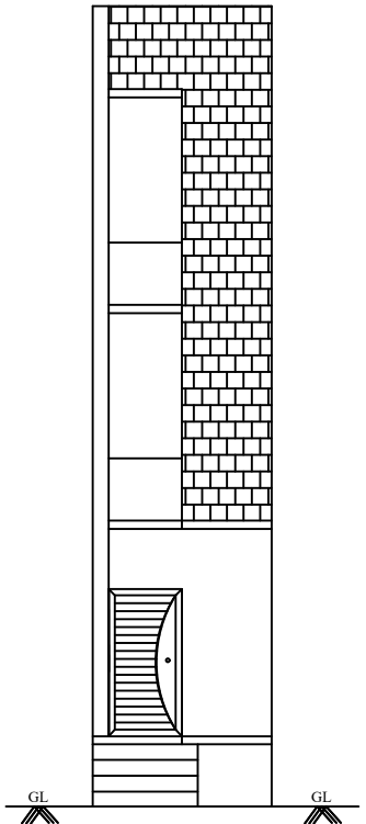
FRONT ELEVATION
