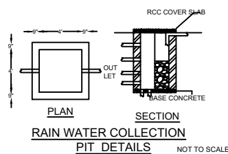
RAIN WATER COLLECTION PIT DETAILS
