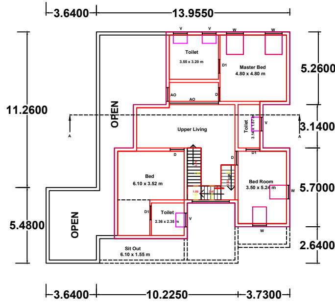
FIRST FLOOR PLAN & OPEN TERRACE
