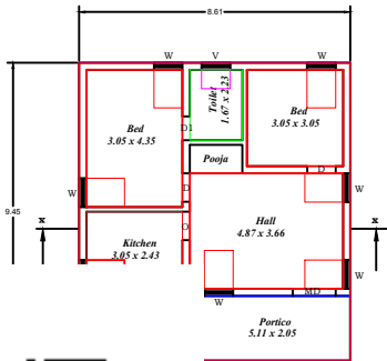
Ground Floor Plan facing
