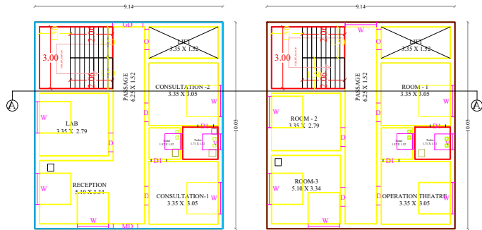
GROUND FLOOR PLAN (WEST FACING)
