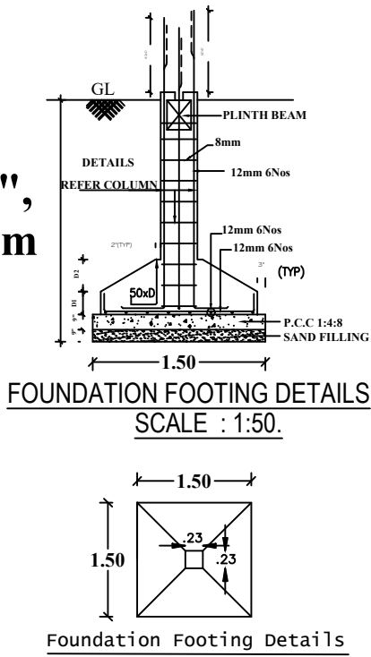
Foundation Footing Details
