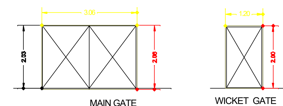
GATE DETAILS
