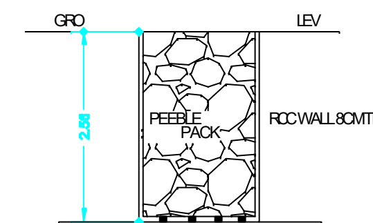
RAIN WATER SUMP DETAILS..
