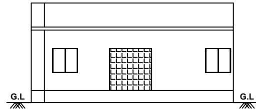
FRONT ELEVATION "A"
