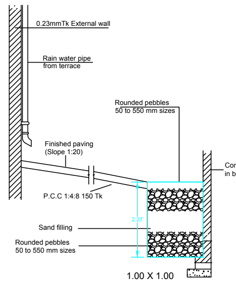
PLAN OF RAIN WATER HARVESTING
