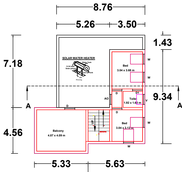
FIRST FLOOR PLAN & TERRACE FLOOR PLAN
