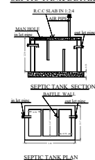
SEPTIC TANK PLAN
