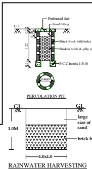
RAINWATER HARVESTING
