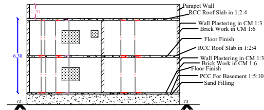
SECTION OF AA
