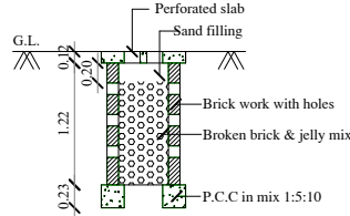
PERCOLATION PIT
