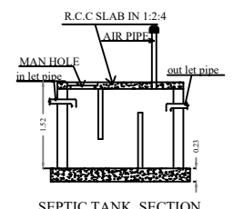
SEPTIC TANK SECTION
