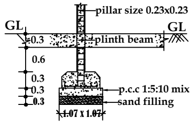
FOUNDATION DETAILS
