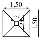
COLUMN FOUNDATION
