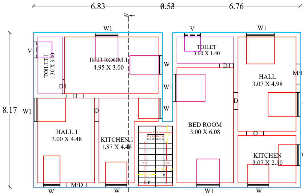
GROUND FLOOR PLAN (SOUTH & EAST FACING)
