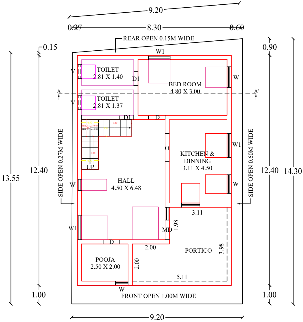
GROUND FLOOR PLAN (SOUTH FACING)
