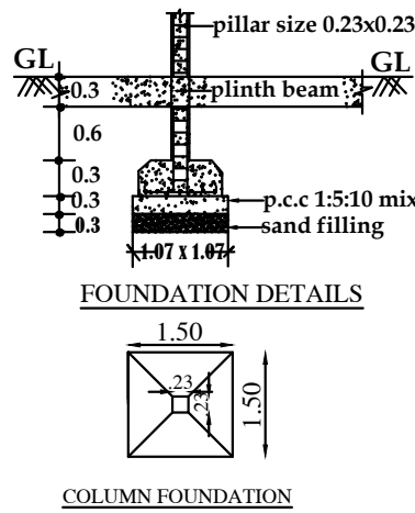
COLUMN FOUNDATION
