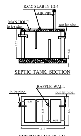
SEPTIC TANK PLAN
