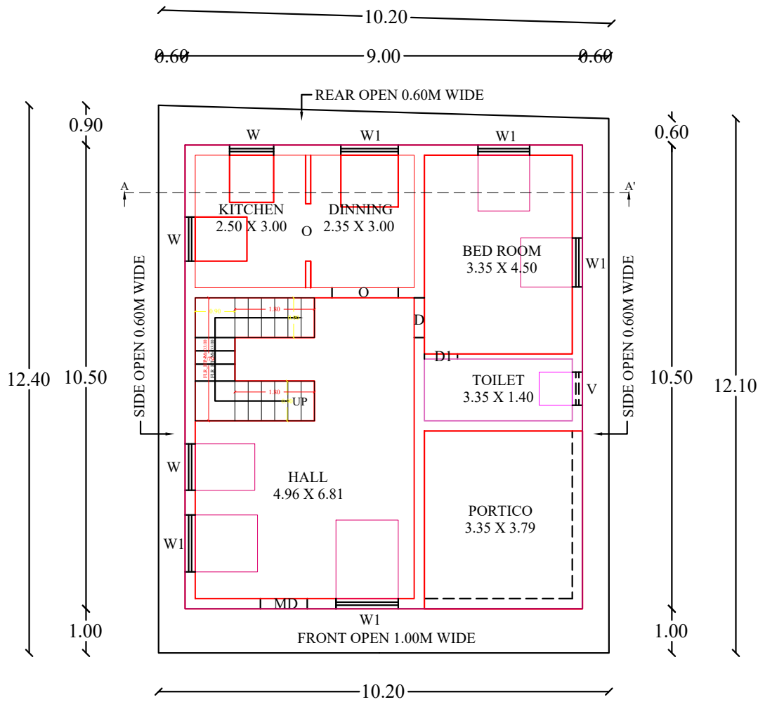
GROUND FLOOR PLAN (NORTH FACING)
