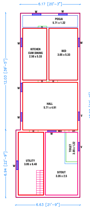
EXISTING GROUND FLOOR PLAN [NORTH FACING]
