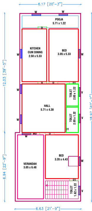
EXISTING & PROPOSED FIRST FLOOR PLAN [NORTH FACING]
