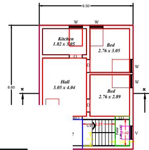
Ground Floor Plan ortho facing
