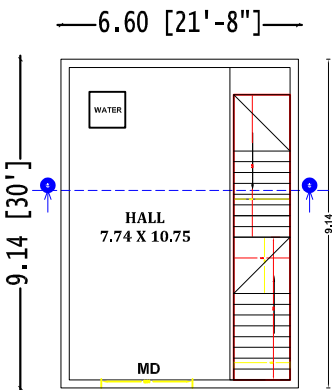
GROUND FLOOR PLAN (NORTH FACING)
