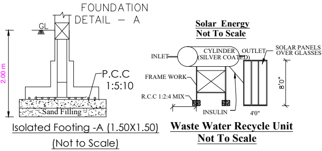
FOUNDATION DETAIL - A
