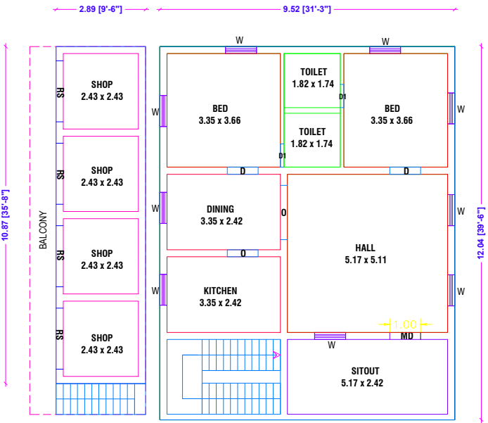
GROUND FLOOR PLAN [ EAST FACING ]
