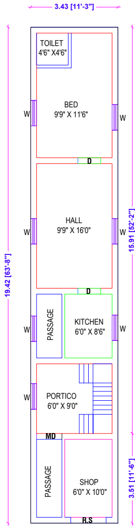
GROUND FLOOR PLAN [ SOUTH FACING ]
