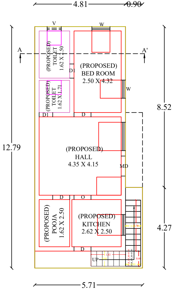
FIRST FLOOR PLAN (PROPOSED BUILDING)
