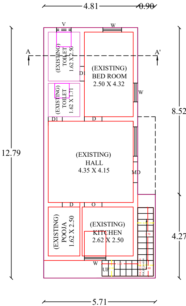
GROUND FLOOR PLAN (EXISTING BUILDING) (EAST FACING)
