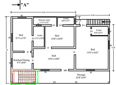
EXISTING GROUND FLOOR PLAN
