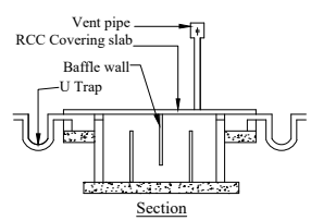
Waste Water Recycle Unit
