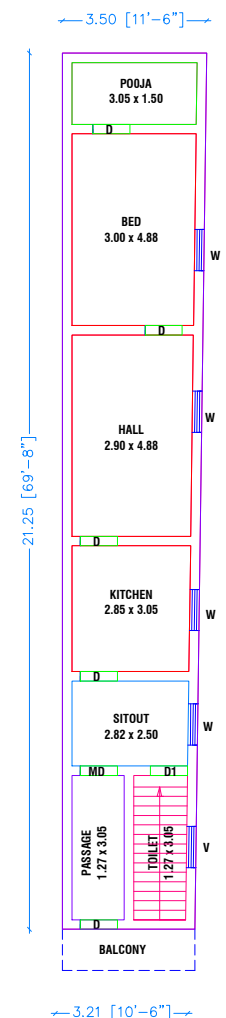
FIRST FLOOR PLAN [SOUTH FACING]
