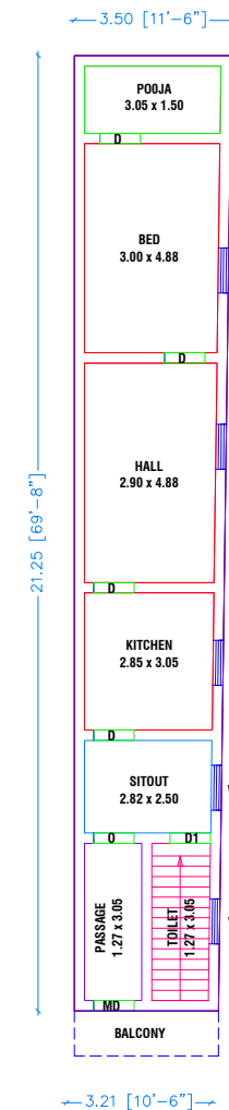
GROUND FLOOR PLAN [SOUTH FACING]
