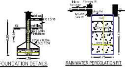
FOUNDATION DETAILS
